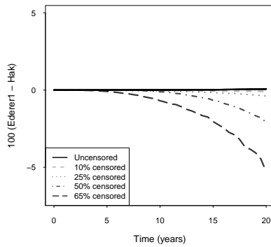
Figure 3: Effect of non-informative censoring on differences between the Ederer I and the Hakulinen estimator (data from Cancer registry of Slovenia, thyroid cancer)
