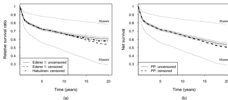
Figure 1: Performance of existing estimators in presence of informative censoring (simulated data) : a) Ederer I and Hakulinen estimator of relative survival ratio, b) PP estimator of net survival. The thin grey curves denote the 95 % confidence intervals for the uncensored case; the dotted curves represent the estimates within the age subgroups.
