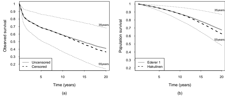
Figure 2: Differences between estimators of the numerator and denominator in the relative survival ratio (simplified example, simulated data) : a) Observed survival, numerator, b) Population survival, denominator. The dotted curves represent the estimates within the age subgroups.
